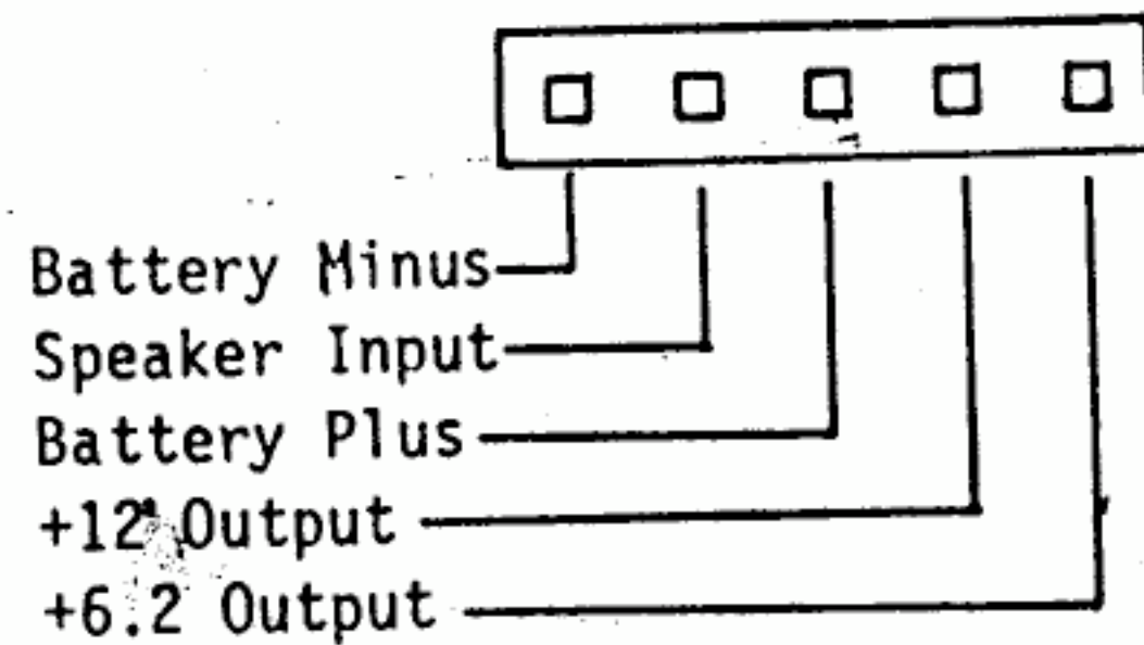
Connector
