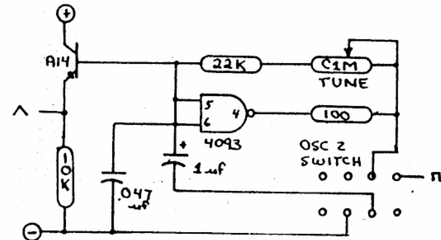
Oscillator 2
